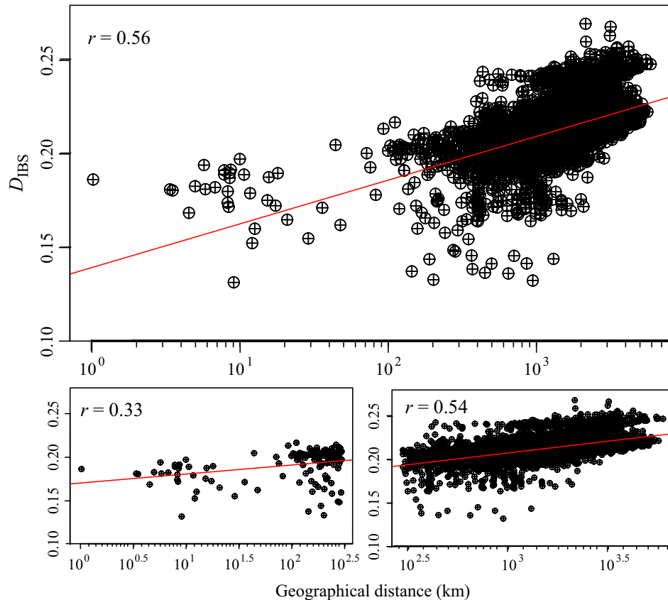
Fig. 3 Isolation by distance for 111 North American wolves and the 42K single-nucleotide polymorphism (SNP) set. Pairwise Genetic distance ( D_{IBS} ) was calculated in PLINK and plotted against the \log_{10} of geographic distance in kilometers for all samples (top panel), individuals closer than 300 km (bottom left panel) and individuals further than 300 km (bottom right panel).
