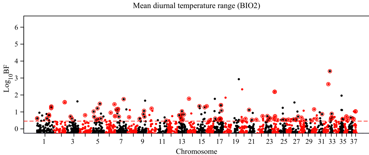
Fig. 6 Manhattan plot of \log_{10} Bayes Factors for Mean Diurnal Temperature Range (BIO2). The chromosomal locations of all single-nucleotide polymorphisms (SNPs) with \log_{10} Bayes factor (BF) > 0 are plotted. SNPs with BF > 3 and within 10 kb of a gene are circled in red. The empirical 99.5th percentile is plotted (dashed red line).
