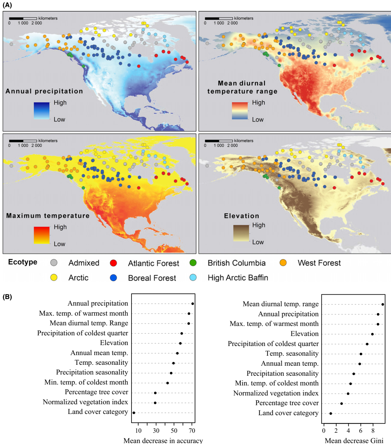
Fig. 2 Environmental variation among wolves sampled in this study. A) Sampling location for wolves imposed on maps of variation for (clockwise, from top left) annual precipitation, mean diurnal temperature range, elevation, and maximum temperature. These variables were ranked as important from Random Forest analysis. B) Output from Random Forest analysis showing which environmental variables were most relevant in assigning individuals to their habitat. Environmental variables with higher mean decrease in accuracy (left) and higher mean decrease in Gini index (right) are shown. See Liaw & Wiener 2002 for details.
