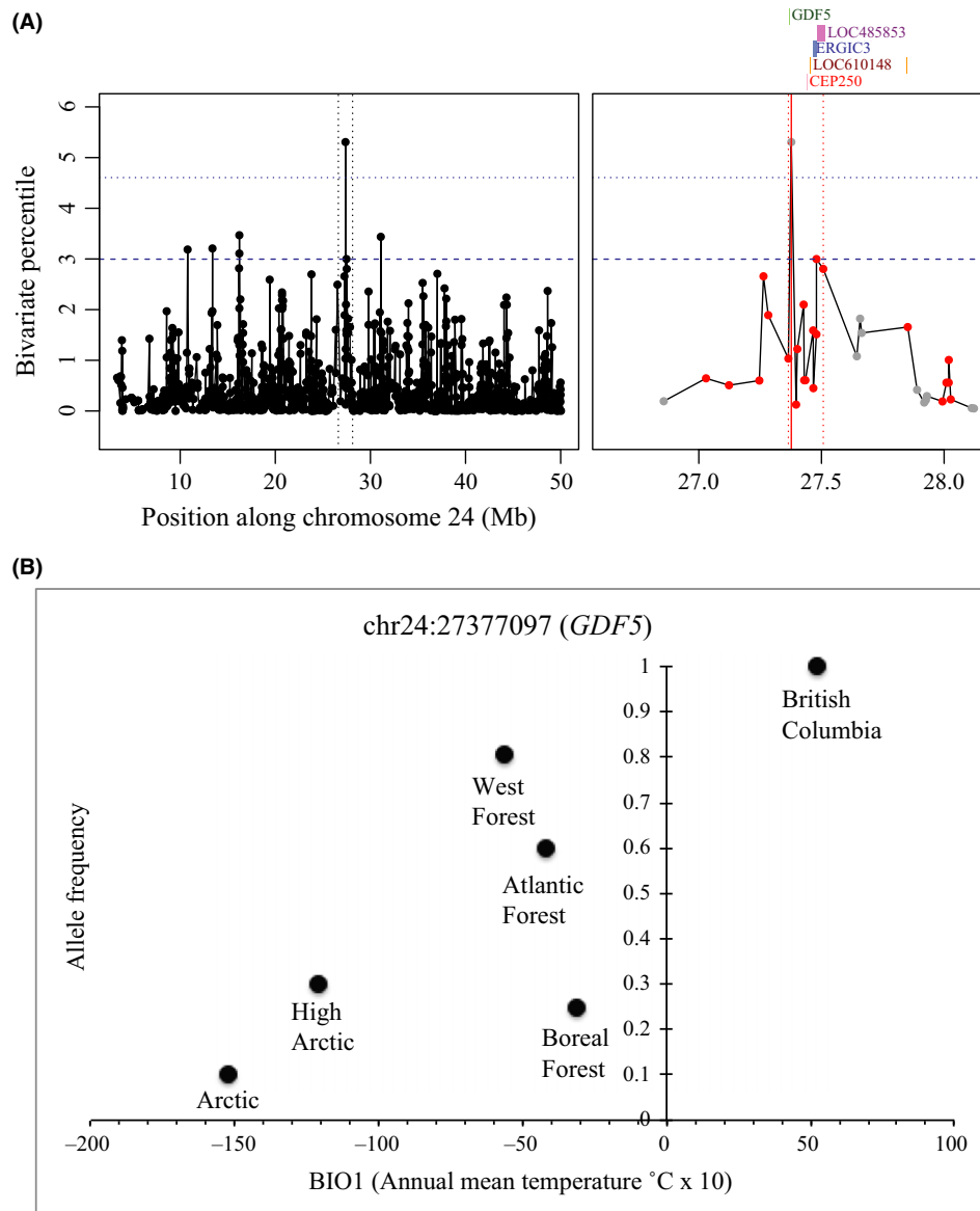
Fig. 4 Signals of selection for Growth Differentiation Factor 5 ( GDF5 ) in Boreal Forest wolves (A) and across all ecotypes (B). A) The bivariate percentile of F_{ST} and XP-EHH for single-nucleotide polymorphisms (SNPs) along Chr 24 in Boreal Forest wolves, with the expanded right panel showing genes overlapping the cluster. B) The annual mean temperature (BIO1, in °C × 10) for each ecotype is plotted along the x-axis, with the mean allele frequency of the SNP tagging GDF5 . SNP location (chromosome and base pair) in Can-Fam2 coordinate is provided.
