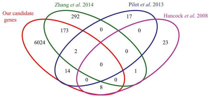
Fig. 7 Venn diagram showing overlap between the union of our candidate genes from F_{ST} /XP-EHH, BAYESCAN, and BAYENV at the 5% significance threshold, and three other studies. The candidate genes from other studies were identified using the Affymetrix canine single-nucleotide polymorphism (SNP) array and BayeScan (Pilot et al. 2013), a scan measuring F_{ST} and nucleotide diversity in whole genome sequences (Zhang et al. 2014), or a seed gene and network approach with tag SNPs and Bayenv (Hancock et al. 2008). Zhang et al. (2014) and Pilot et al. (2013) used wolves as a study system, and Hancock et al. (2008) studied humans.
