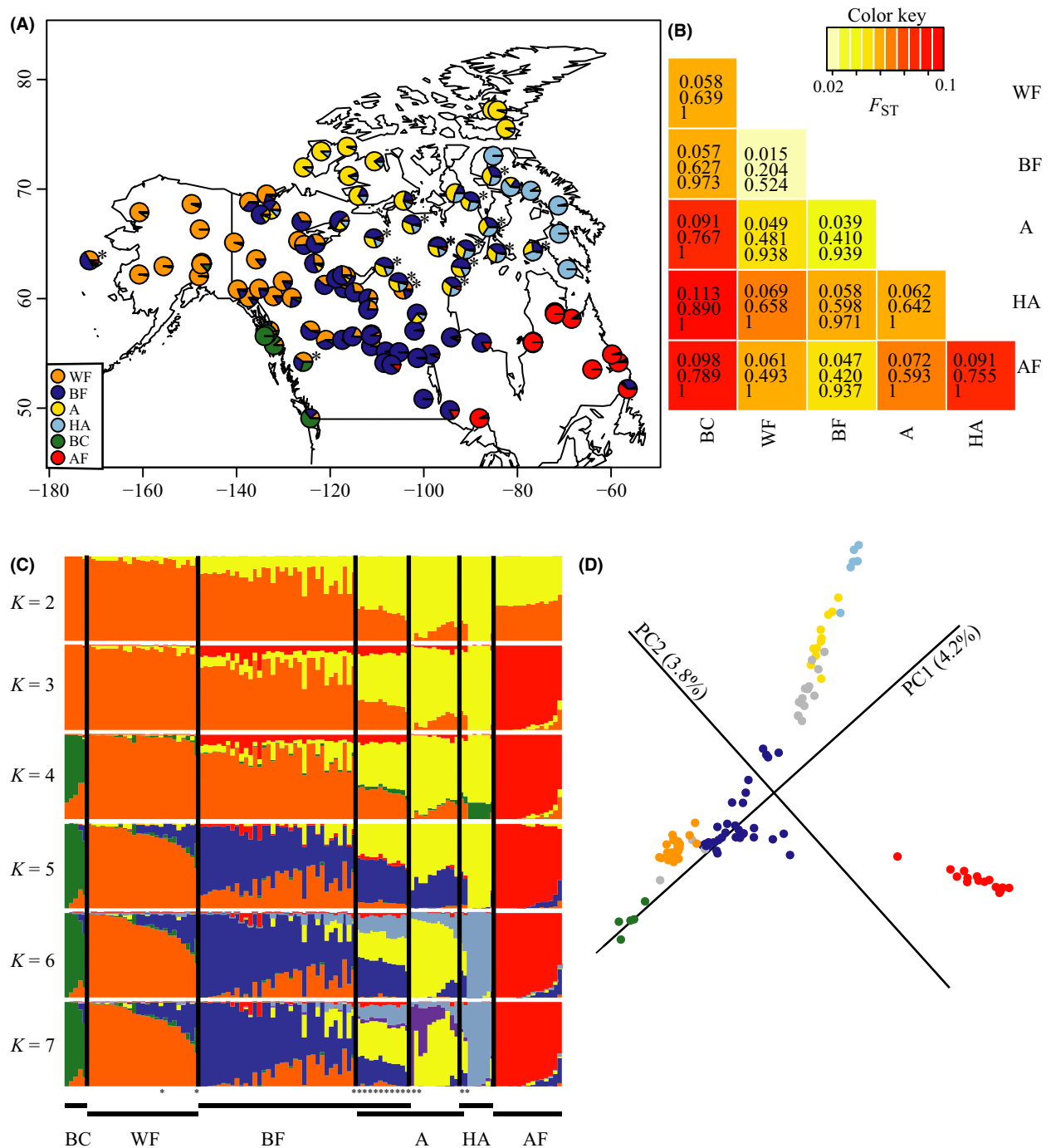
Fig. 1 Genetic differentiation among wolf populations. A) Sampling locations of 111 wolves. Each wolf is symbolized by a pie chart with relative proportion of assignment at K = 6 in STRUCTURE. Individuals with an '*' were admixed at K = 6 and were removed from further analysis. B) Heatmap of pairwise F_{ST} for 42K single-nucleotide polymorphisms (SNPs) in 94 non-admixed wolves. The mean, 99th percentile, and maximum pairwise F_{ST} are labeled from top to bottom. C) STRUCTURE plot for K = 2 to K = 7 . Admixed individuals are marked with an '*'. D) PCA plot of 111 wolves for 22K LD-pruned data set, slightly rotated to match map in A). Colors represent STRUCTURE groupings, with admixed/removed individuals in gray. WF: West Forest, BF: Boreal Forest, A: Arctic, HA: High Arctic, BC: British Columbia, AF: Atlantic Forest.
